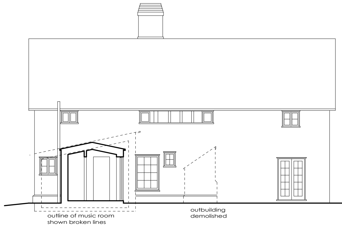
section through link/ west elevation
