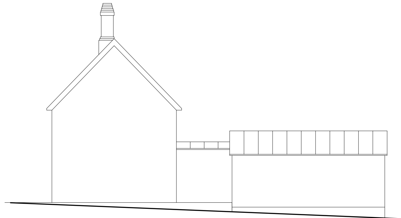
south elevation
